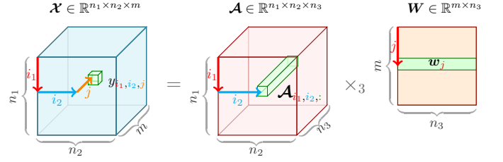
Fig. 4. Illustration of the modal product between a third-order tensor and a matrix. By definition, the entry of resulting tensor \mathcal{X} is the inner product between tensor fiber (i.e., in the form of a vector) of \mathcal{A} and row vector of \mathbf{W} [29], [30].
