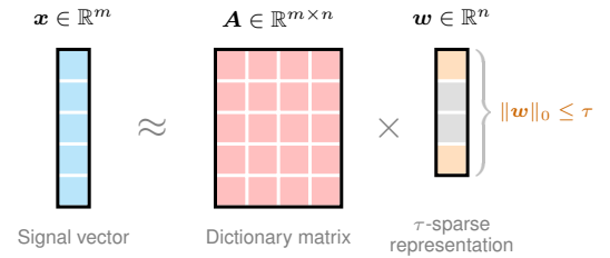
Fig. 2. Linear regression problem \min_{\mathbf{w}} \|\mathbf{x} - \mathbf{A}\mathbf{w}\|_2^2 with \tau -sparse representation of the coefficient vector \mathbf{w} . In compressive sensing, the goal is to construct a sparse vector \mathbf{w} given measurements \mathbf{x} (i.e., the signal) and \mathbf{A} (e.g., the dictionary) [13]. The vector \mathbf{w} is constrained to have no more than \tau non-zero entries in which \tau \in \mathbb{Z}^+ refers to the sparsity level.
