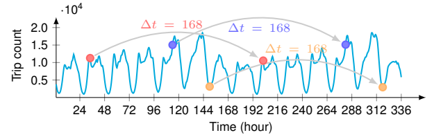
Fig. 1. Hourly ridesharing trip time series in Chicago during the first two weeks since April 1, 2024. The time series exhibits weekly seasonality as \Delta t = 168 .
