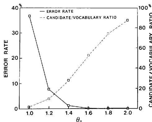
Fig. 5. Preprocessor performance for Method B-1: preselection by unbiased distance threshold.
