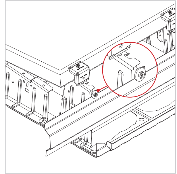
STEP 3 - HARDWARE: Secure wind deflector with 1 ½" O.D. flat washer and ¼-20 x 1" Bolt, as shown above
