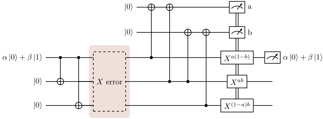
Figure 13.7: The quantised version of the classical [3, 1, 3] code. If at most one bit-flip error occurs in the shaded region (which denotes the part where we transmit over a noisy channel), then this circuit perfectly corrects it, resulting in the successful transmission of the state \alpha|0\rangle + \beta|1\rangle .
