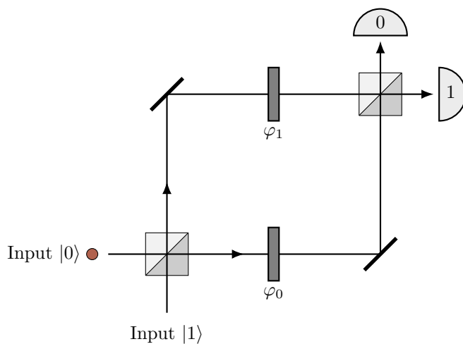
Figure 3.5: The Mach-Zehnder interferometer , with the input photon represented by the coloured dot. This experimental set-up is named after the physicists Ludwig Mach and Ludwig Zehnder , who proposed it back in 1890s.
