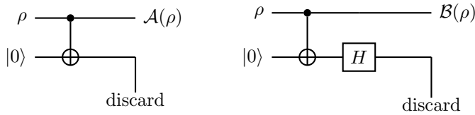
Figure 9.2: The c-NOT gate appears here as the measurement gate. The target qubit (on the bottom) measures the control qubit (on the top) in the standard basis (operation \mathcal{A} on the left) or in the Hadamard basis (operation \mathcal{B} on the right). The extra Hadamard gate on the target qubit has no effect on the control qubit.
