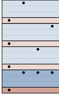
Figure 14.13: All computational errors of weight at most 1 for the three-qubit code given by \langle ZZ1, 1ZZ \rangle . Note that this describes a non -correctable scenario. In fact, both of the two rules are broken.
