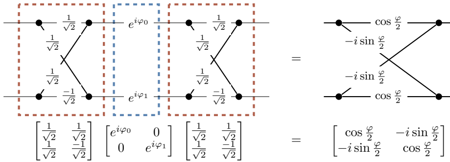
Figure 1.3: The Ramsey interferometer represented as an abstract diagram (matrix approach). Here we have omitted the |0\rangle and |1\rangle labels, just to simplify the diagram. We also ignore (for reasons that we will later explain) the global phase factor of e^{i\frac{\varphi_0+\varphi_1}{2}} .
