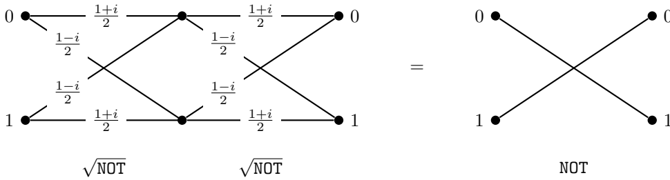
Figure 2.2: A computation that, when repeated, gives exactly NOT. An unlabelled line means that it has probability 1, and the lack of a line corresponds to having probability 0.
