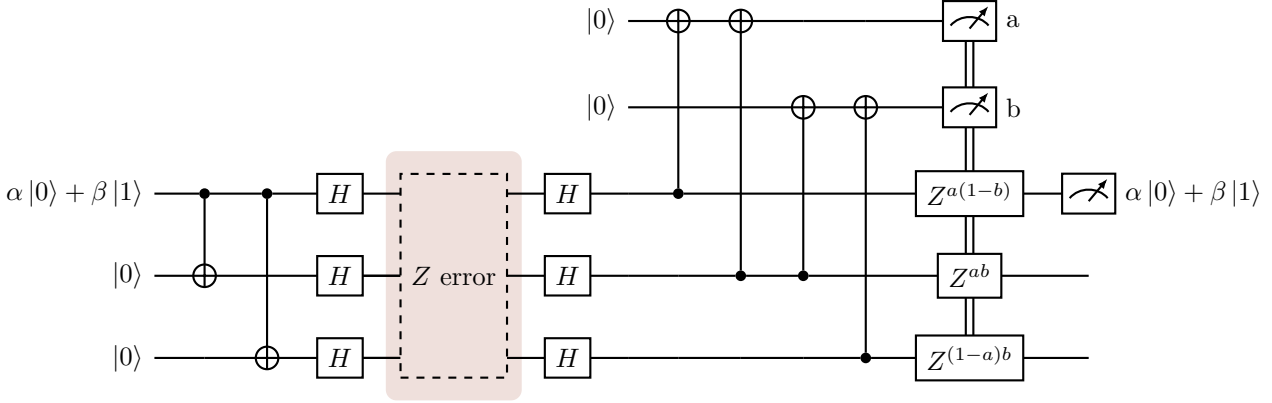
Figure 13.8: Using the quantised [3, 1, 3] code to deal with phase-flips by sandwiching the transmission area between Hadamards.
