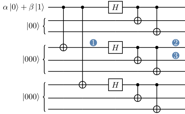
Figure 13.9: The encoding circuit for the Shor [[9, 1, 3]] code, implementing (V_{00} \otimes V_{00} \otimes V_{00})(H \otimes H \otimes H)V_{00} . The three locations marked with numbers are not part of the circuit, but we will use them to explain how this circuit corrects for arbitrary single-qubit errors.
