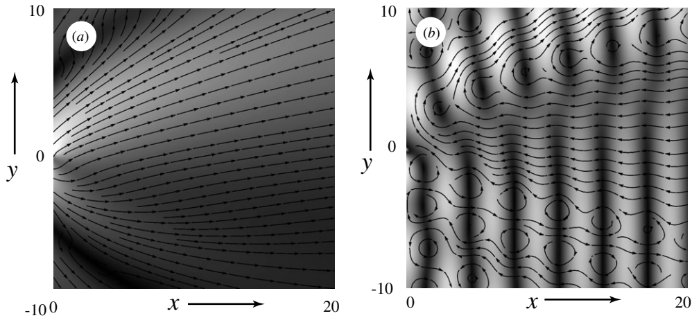
Figure 6. (a) Scattered wave \psi_{sc} = \psi - 2\cos x (equation 5.14) in reflection from a Dirichlet singularity, for \varepsilon = 1 , \mu = \arg A = 0 , showing |\psi_{sc}| as a density plot (with lighter shading representing higher intensity), and streamlines of the current vector \text{Im} \psi_{sc}^* \nabla \psi_{sc} . (b) As (a), for the total wave \psi .
