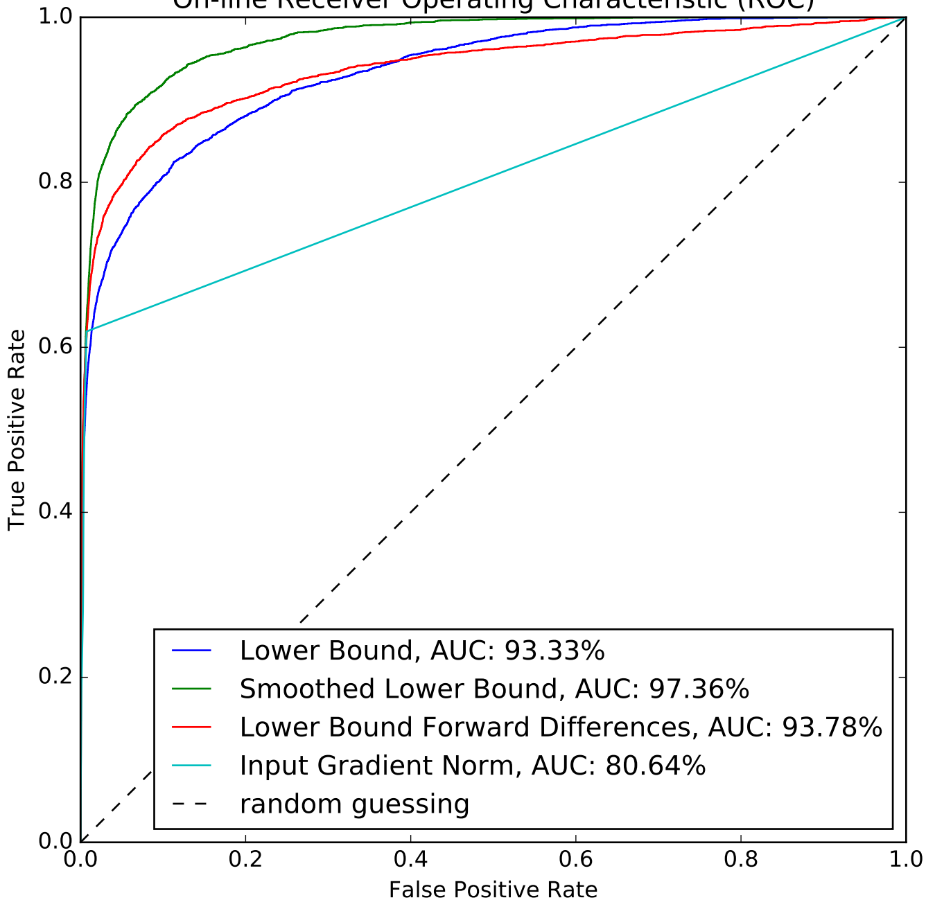
On-line Receiver Operating Characteristic (ROC)
