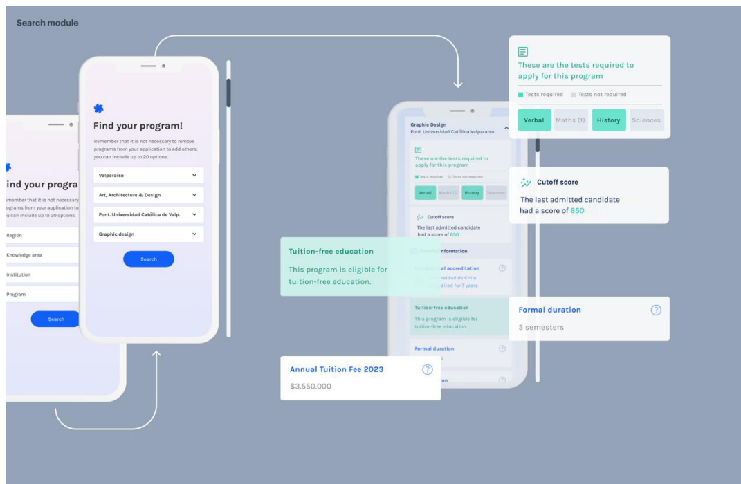
Figure 7: Search module
