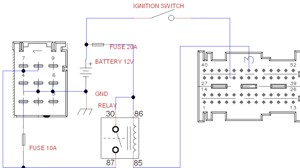
Figure 2.2: Correct power supply wiring for controllers with serial numbers 200 and up. This is not optional. You can not alter this in any way. Do not use a PDM. Do not use a battery cut off switch to interrupt the feed to this relay. If it is even remotely possible to interrupt power to the ECU while the engine is running, there is a risk of fuel system damage as the rail pressure must be regulated while pump is turning.
