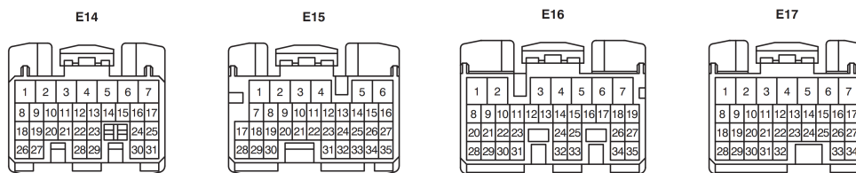
Figure J.1: OEM ECU connectors, as seen looking into the end that mates with the ECU. Connector A=E14, B=E15, C=E16, D=E17
